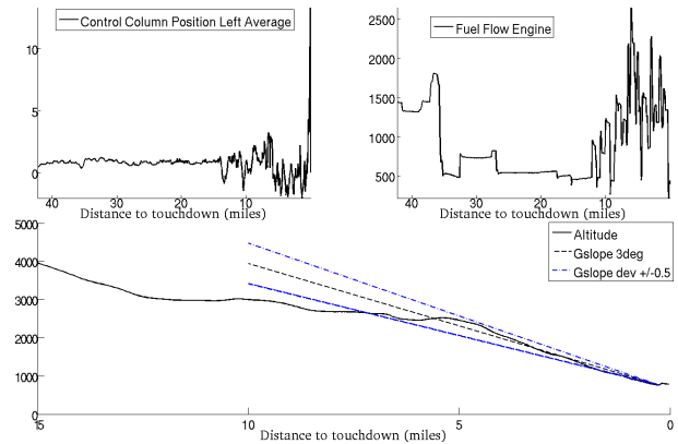
Figure 8: Top anomalous parameters associated with the abnormal approach anomaly. The top left plot shows the high control column position. The top right plot shows the large swings in fuel flow activity. The bottom plot shows the altitude vs. the distance to landing with the glide slope and glide slope deviation superimposed.
