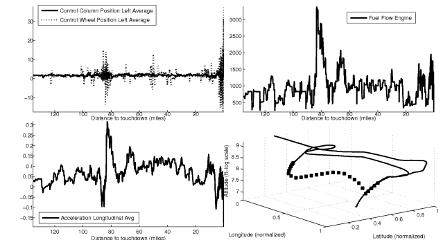
Figure 5: Top anomalous parameters associated with a go-around. The top left plot shows the control column and wheel positions associated with the maneuver. The top right plot shows high fuel flow consumption related to the climb. The bottom left plot shows the high acceleration in the longitudinal direction. The bottom right plot shows the 3 dimensional track of the aircraft (the go-around maneuver is denoted by the dotted lines)
