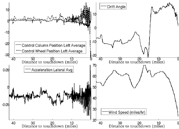
Figure 7: Top anomalous parameters associated with the gusty wind anomaly. The top left plot shows the control column and wheel positions. The top right plot shows the high drift angle. The bottom left plot shows high lateral (side-to-side) accelerations. The bottom right plot shows the wind speed gusts.
