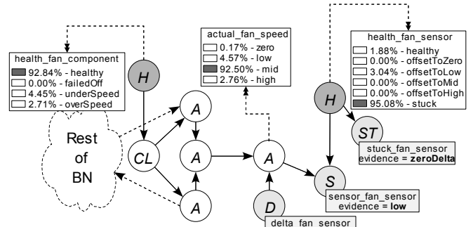
Figure 7: The marginal distributions for health H nodes health\_fan\_component and health\_fan\_sensor as well as the actual\_fan\_speed attribute A node, when the stuck ST node is clamped to the stuck state.
