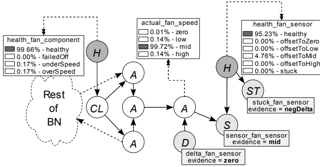
Figure 5: The marginal distributions for health H nodes health\_fan\_component and health\_fan\_sensor as well as the actual\_fan\_speed attribute A node (same representation as in Figure 2). The actual\_fan\_speed A node represents the actual state of the fan's blades.
