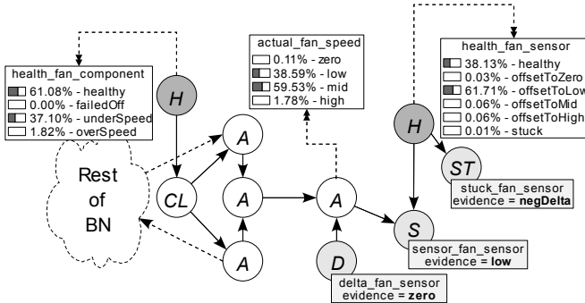
Figure 6: The marginal distributions for health H nodes health\_fan\_component and health\_fan\_sensor as well as the actual\_fan\_speed attribute A node, when the fan sensor's evidence (sensor reading - state) is changed to low.
