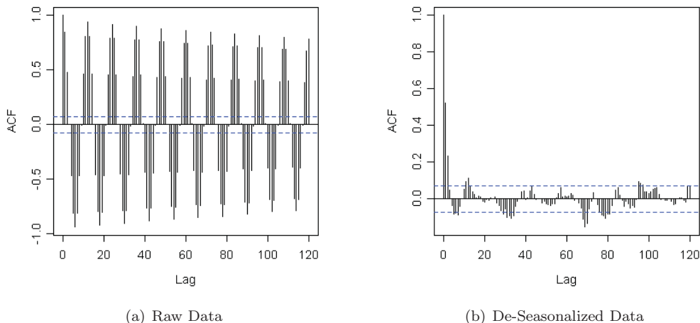
FIGURE 2. The de-seasonalized data (right) exhibits significantly lower autocorrelation due to seasonality than the raw data (left).
