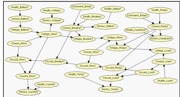
Figure 2: Auto-generation of a Bayesian network representing an electrical power system (bottom) from a high-level system specification (top).
