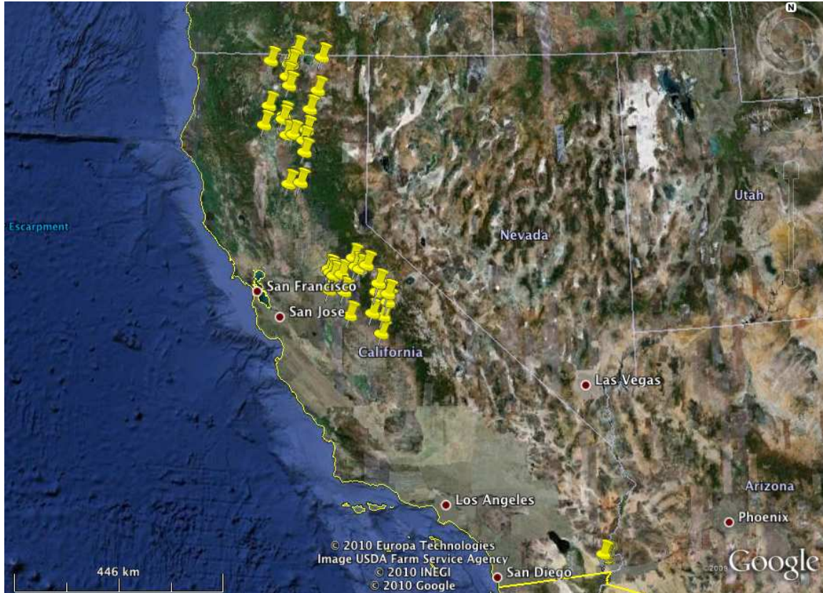
FIGURE 9. Top 50 outliers detected by the distributed algorithm but not detected by the first site using its data only. This is for training set size of 100,000.
