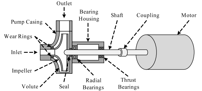
Figure 3. Centrifugal pump.
