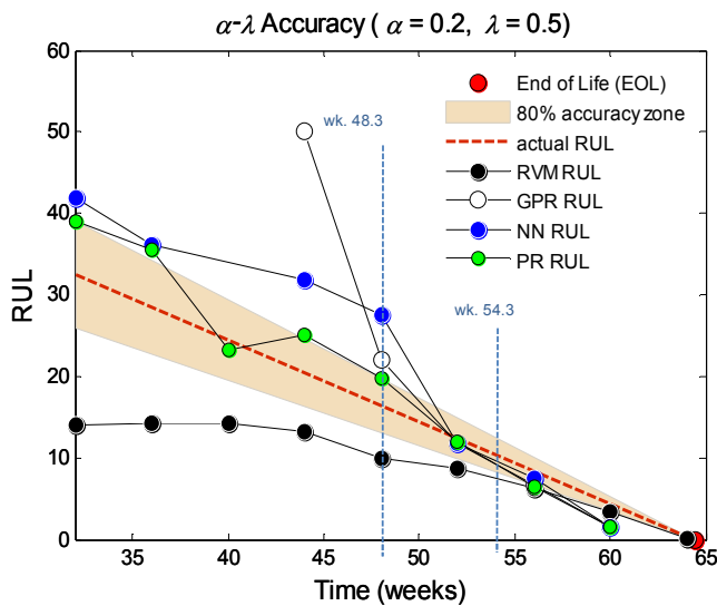
Figure 7 – The \alpha - \lambda Accuracy metric determines whether predictions are within the cone of desired accuracy levels at a given time instant ( t_{\lambda} ).
