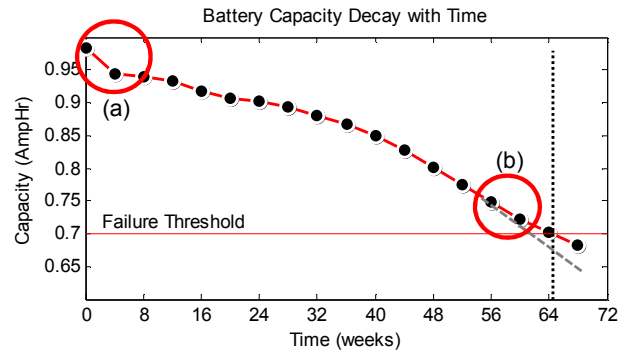
Figure 8 – Battery capacity decay profile shows several features that are difficult to learn using simple regression techniques.
